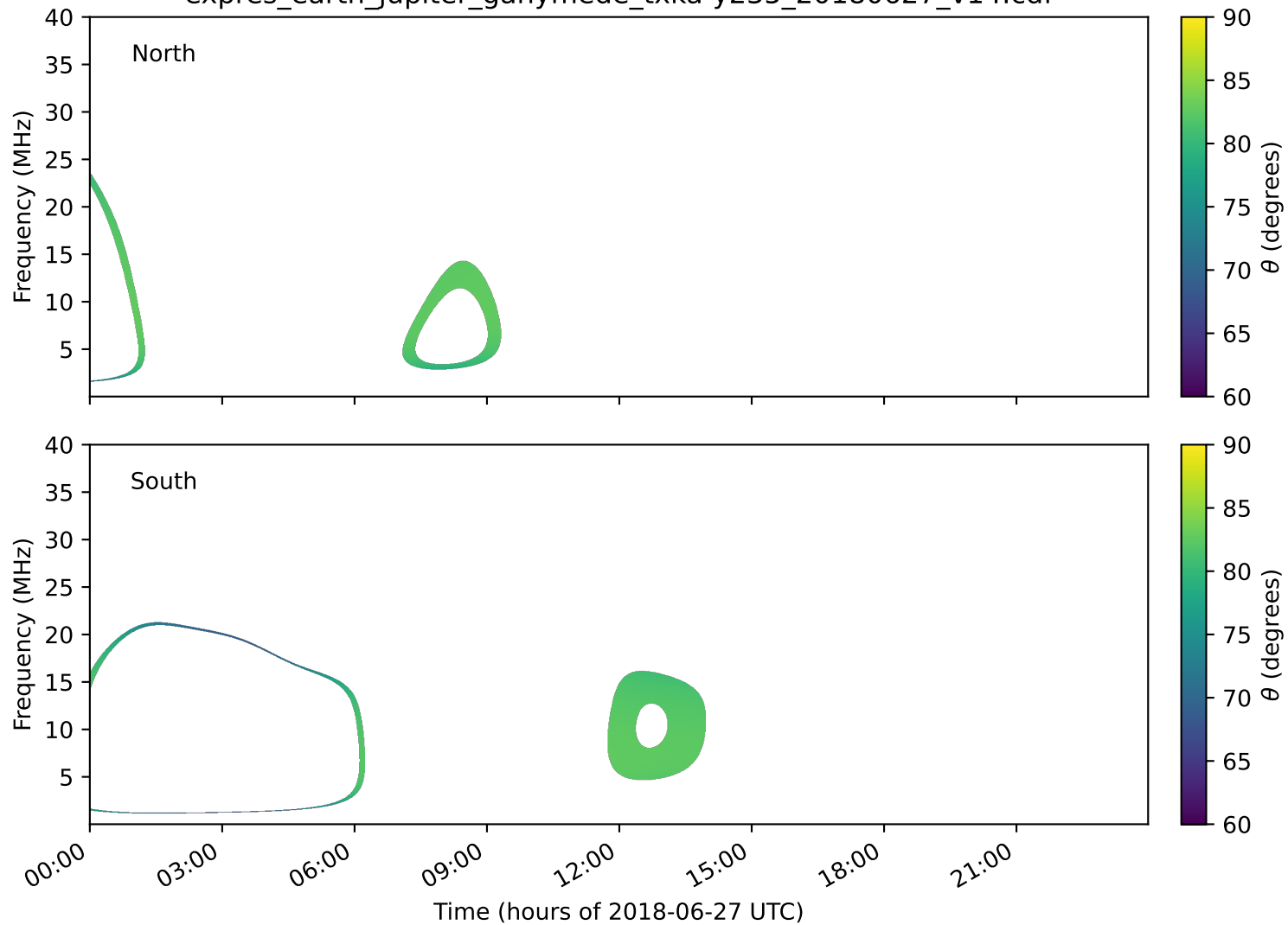
expres_earth_jupiter_ganymede_txka-y235_20180627_v14.cdf
