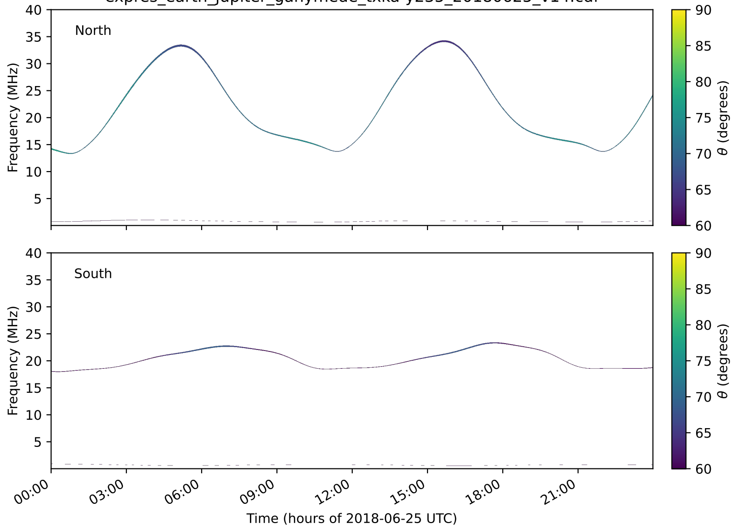
expres_earth_jupiter_ganymede_txka-y235_20180625_v14.cdf
