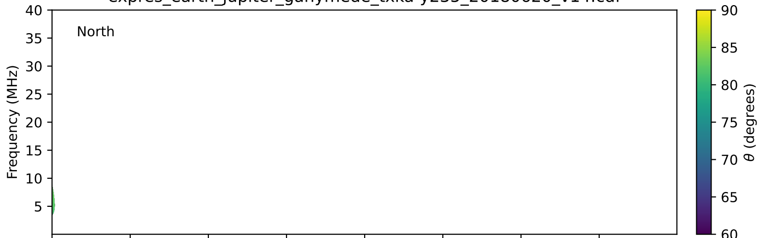
expres_earth_jupiter_ganymede_txka-y235_20180620_v14.cdf
