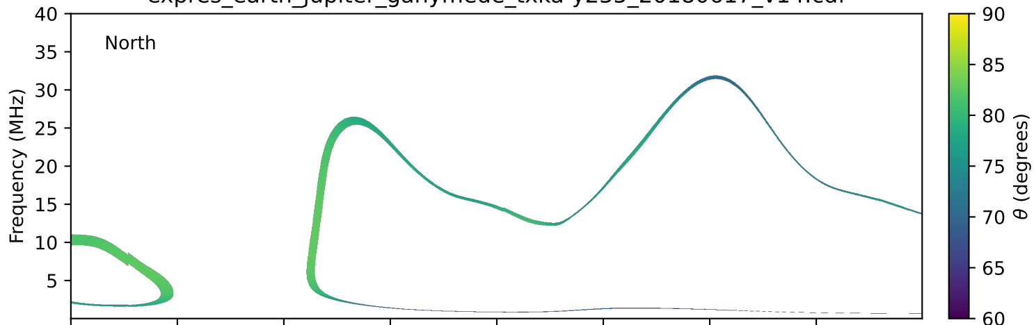
expres_earth_jupiter_ganymede_txka-y235_20180617_v14.cdf
