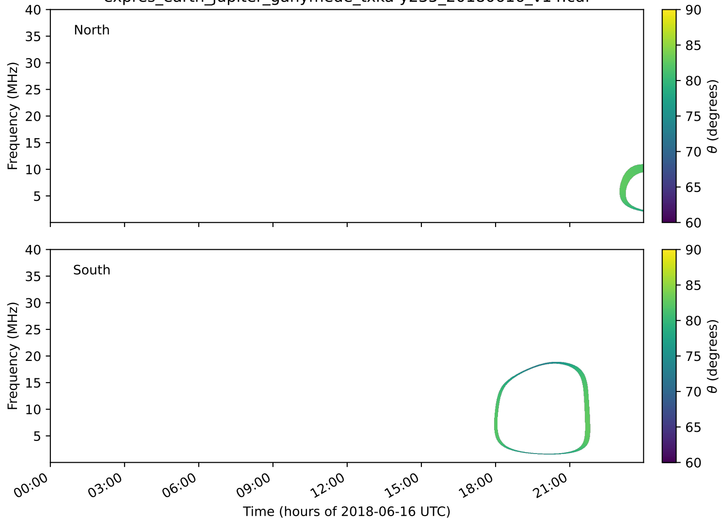
expres_earth_jupiter_ganymede_txka-y235_20180616_v14.cdf
