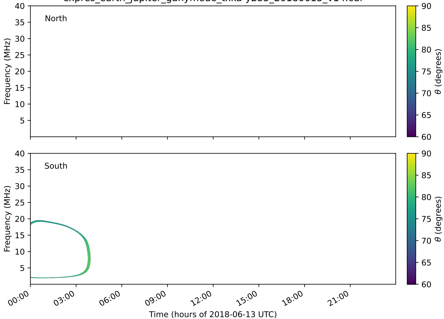
expres_earth_jupiter_ganymede_txka-y235_20180613_v14.cdf
