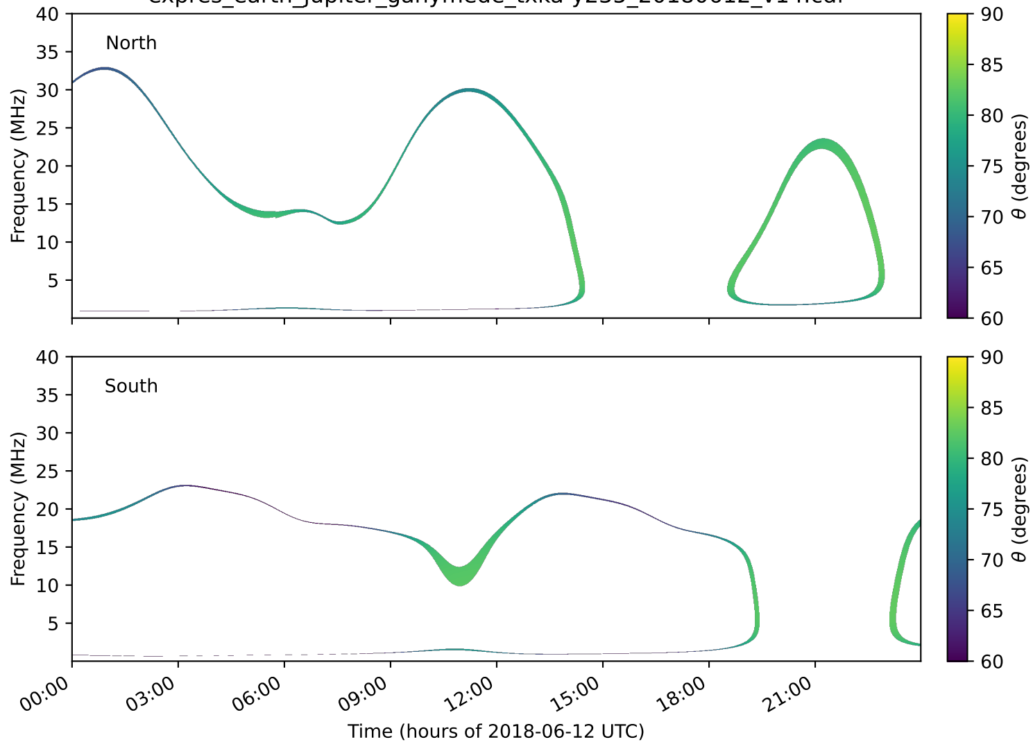
expres_earth_jupiter_ganymede_txka-y235_20180612_v14.cdf
