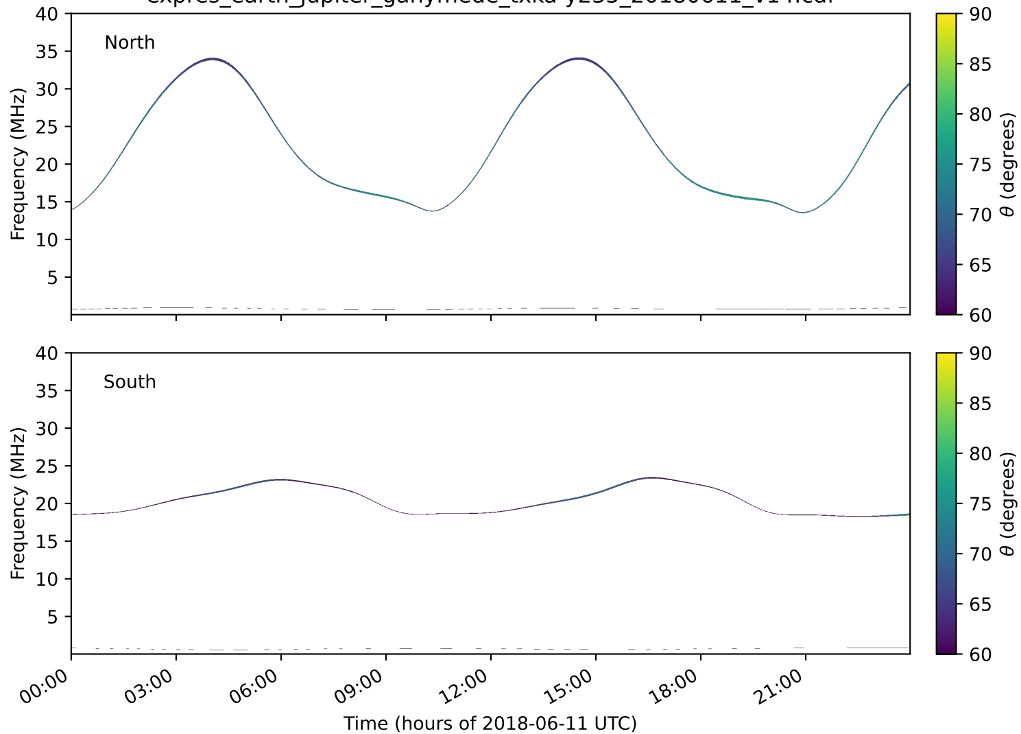
expres_earth_jupiter_ganymede_txka-y235_20180611_v14.cdf
