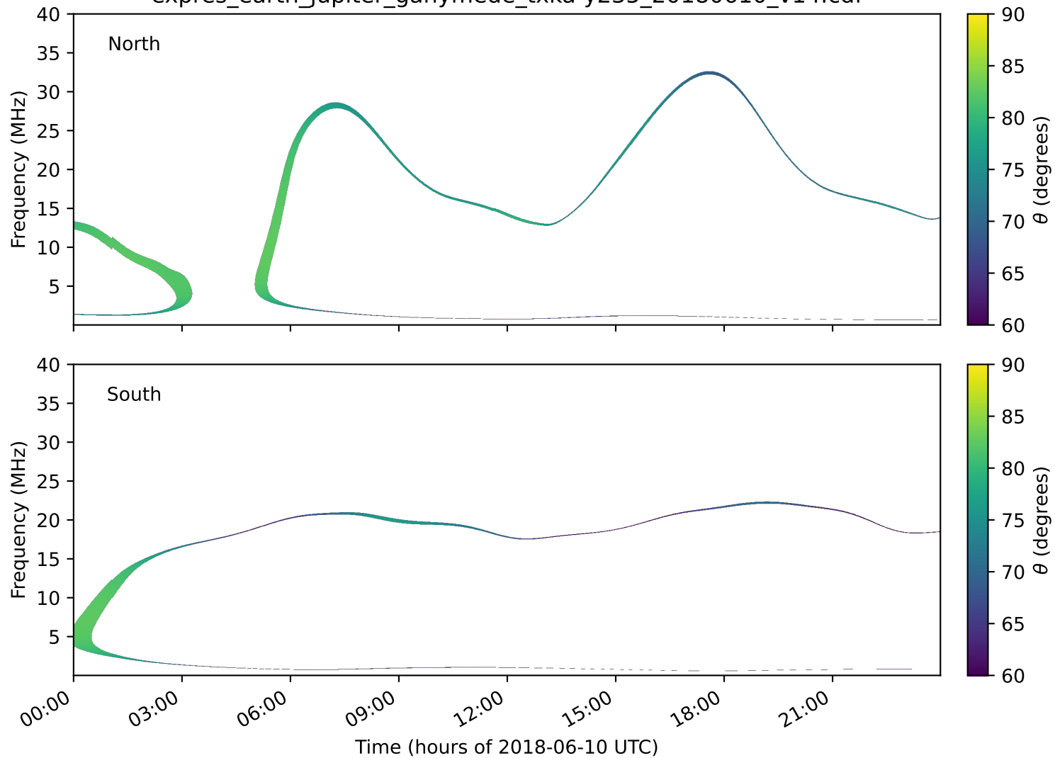
expres_earth_jupiter_ganymede_txka-y235_20180610_v14.cdf
