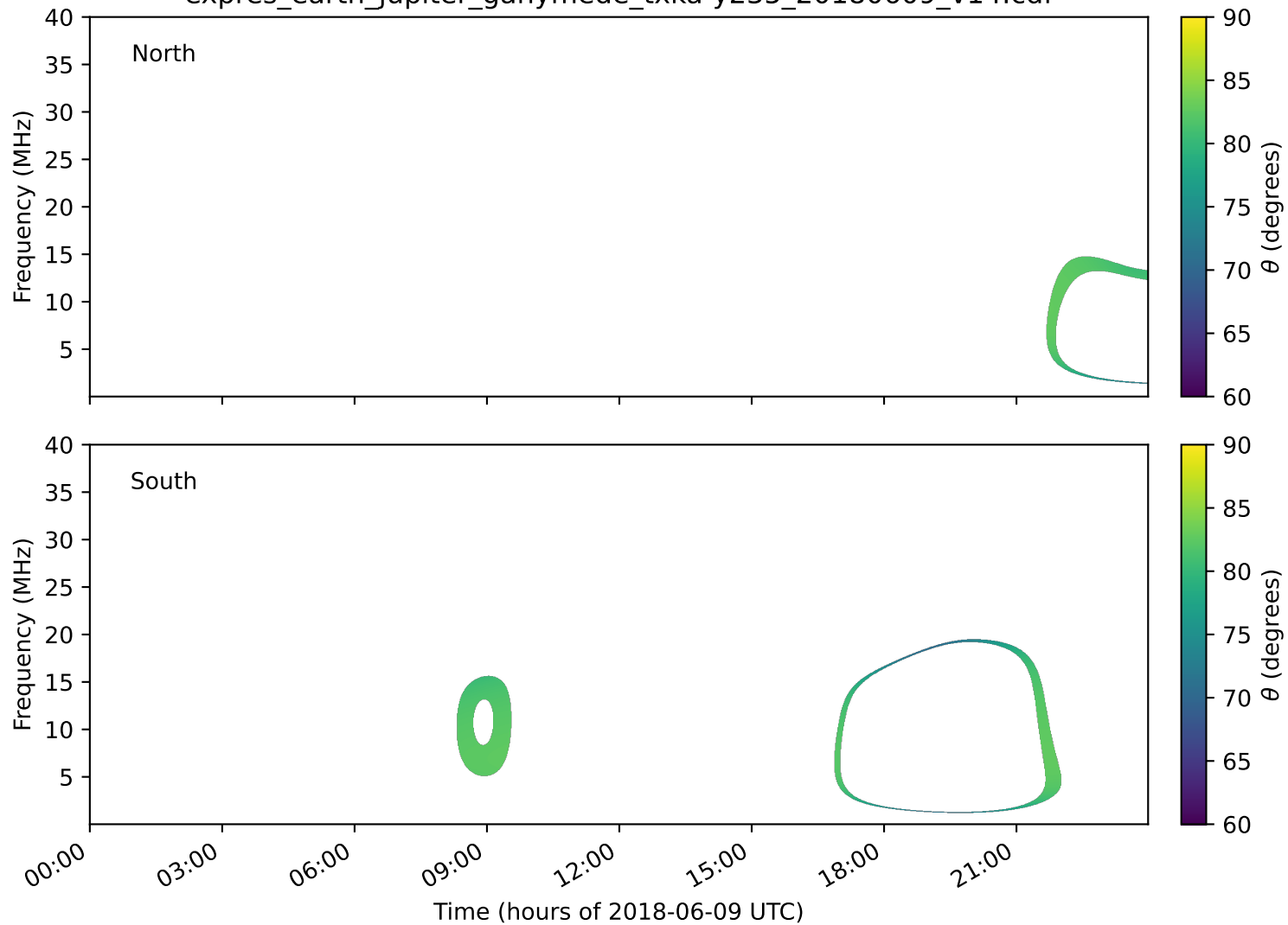
expres_earth_jupiter_ganymede_txka-y235_20180609_v14.cdf
