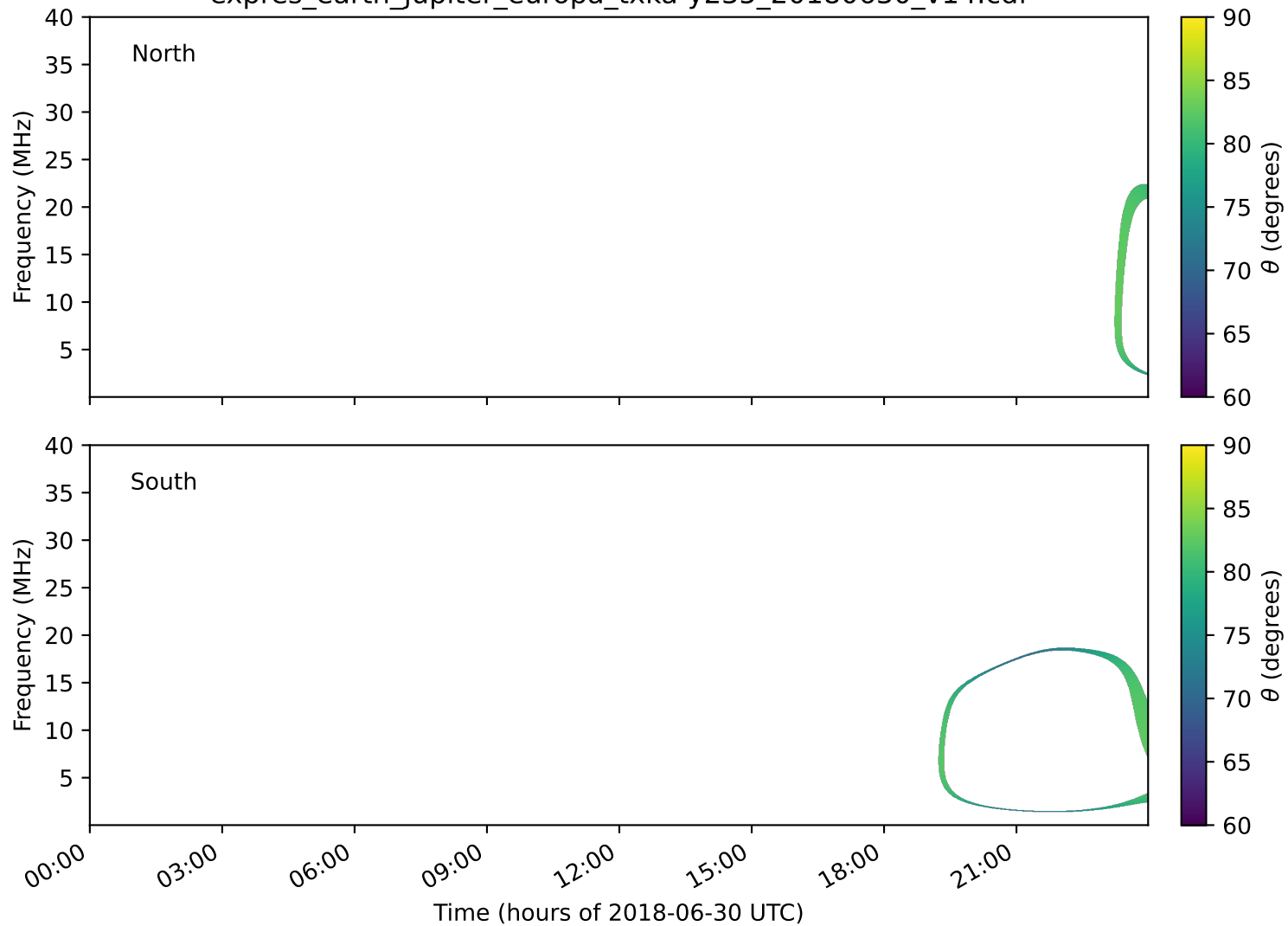
expres_earth_jupiter_europa_txka-y235_20180630_v14.cdf
