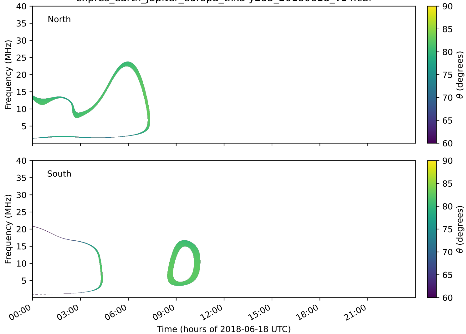
expres_earth_jupiter_europa_txka-y235_20180618_v14.cdf
