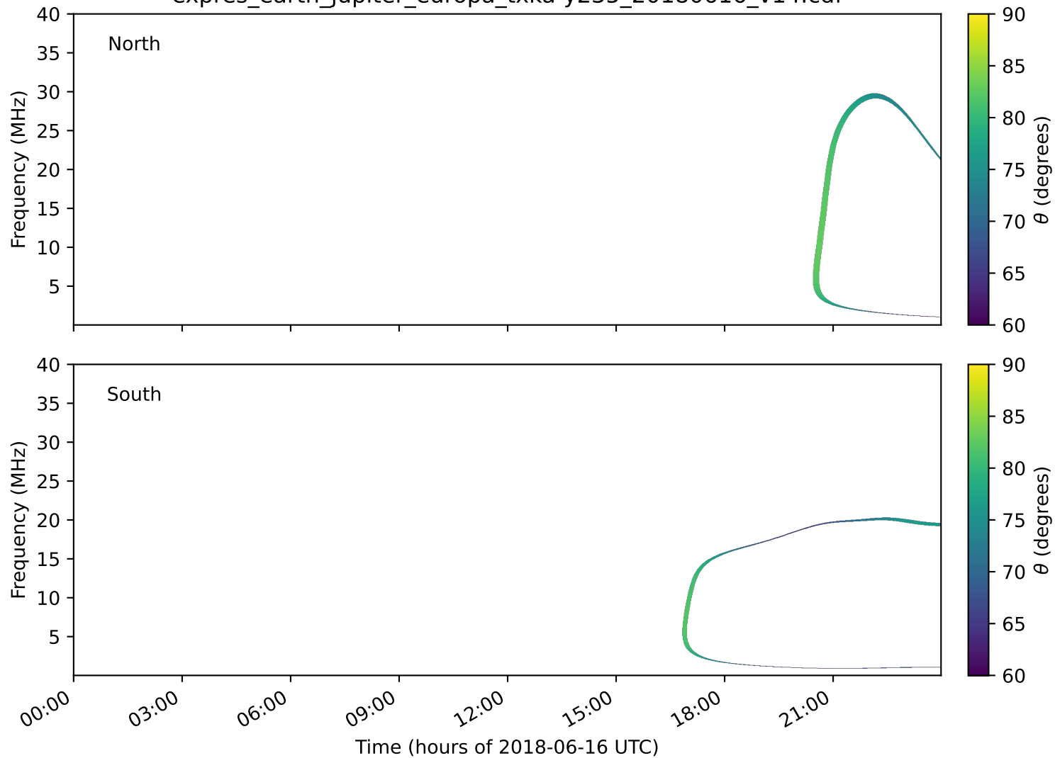
expres_earth_jupiter_europa_txka-y235_20180616_v14.cdf
