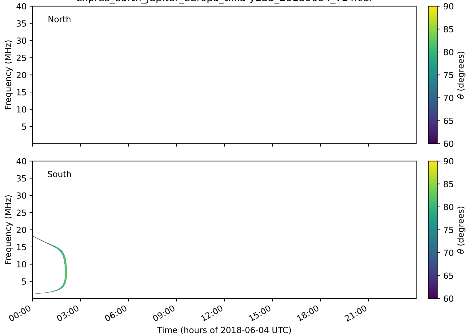
expres_earth_jupiter_europa_txka-y235_20180604_v14.cdf
