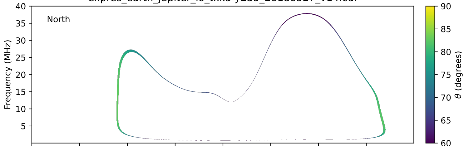
expres_earth_jupiter_io_txka-y235_20180527_v14.cdf
