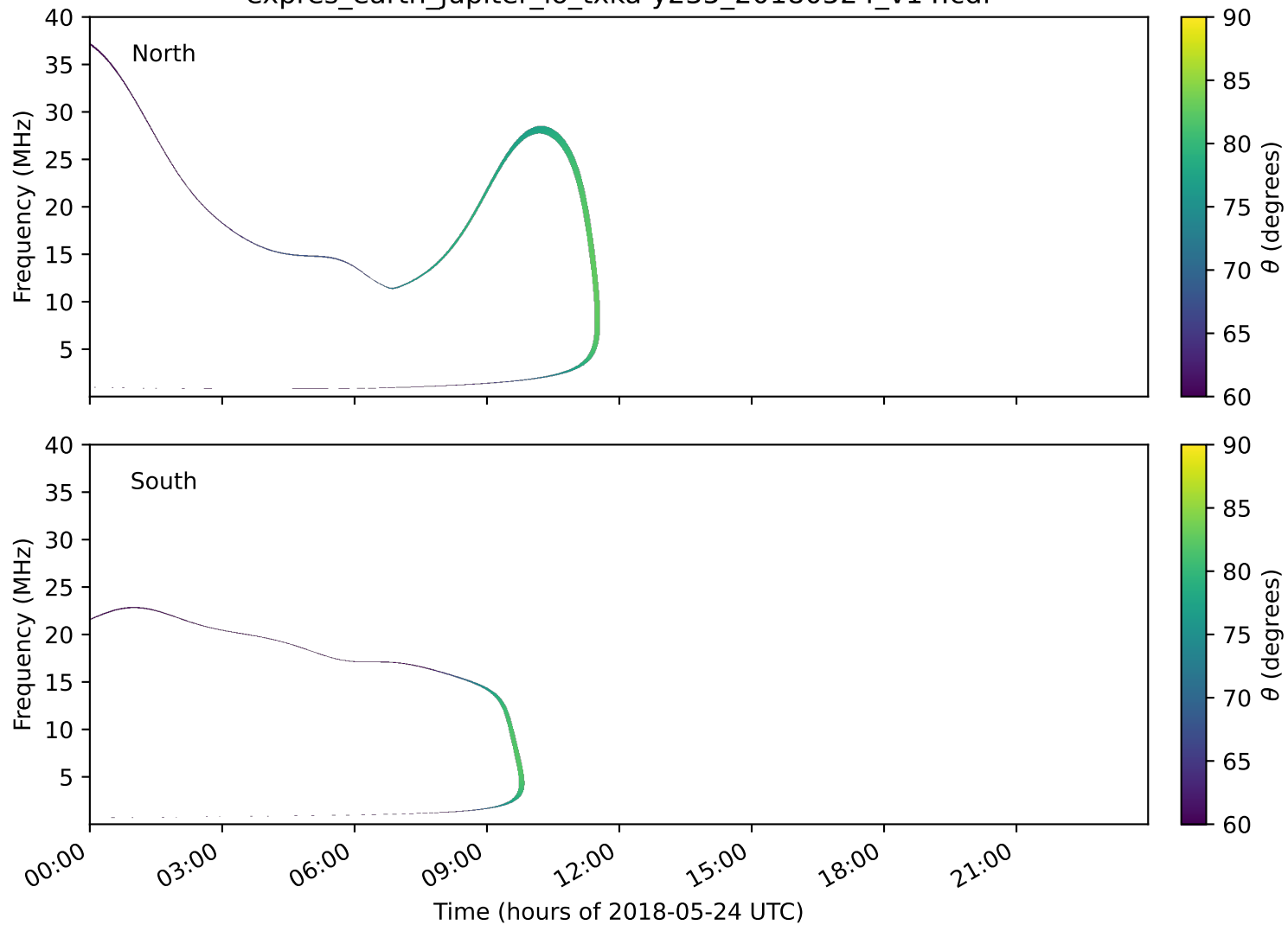
expres_earth_jupiter_io_txka-y235_20180524_v14.cdf
