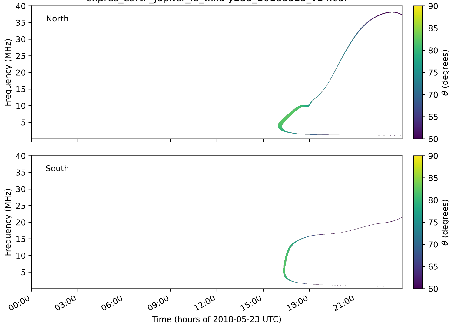
expres_earth_jupiter_io_txka-y235_20180523_v14.cdf
