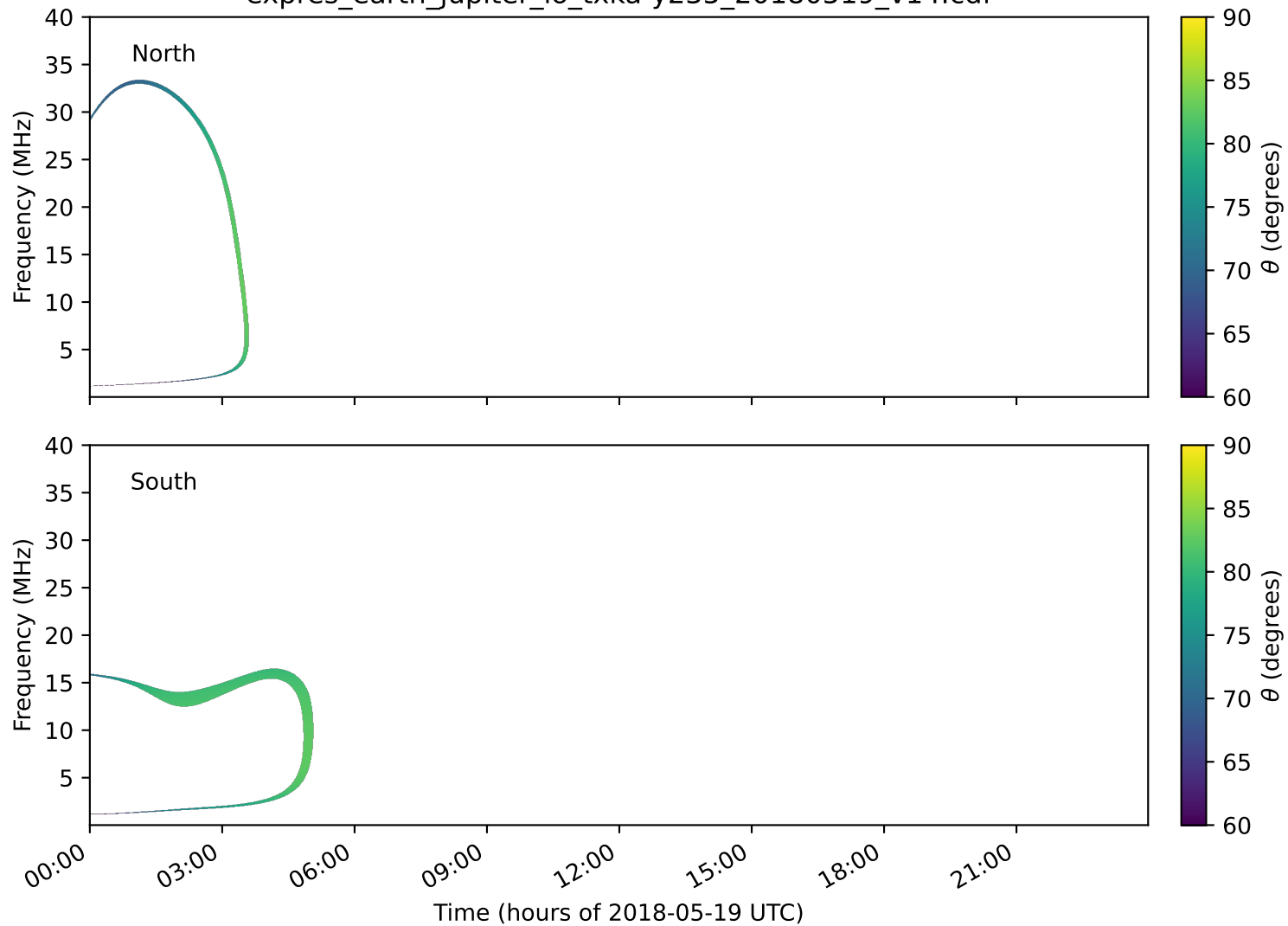
expres_earth_jupiter_io_txka-y235_20180519_v14.cdf
