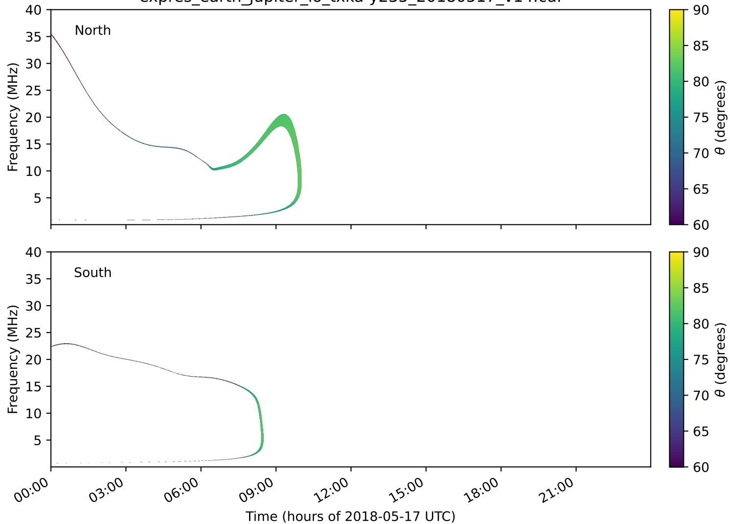
expres_earth_jupiter_io_txka-y235_20180517_v14.cdf
