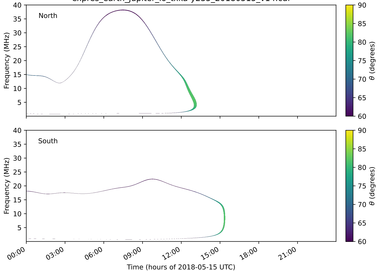
expres_earth_jupiter_io_txka-y235_20180515_v14.cdf
