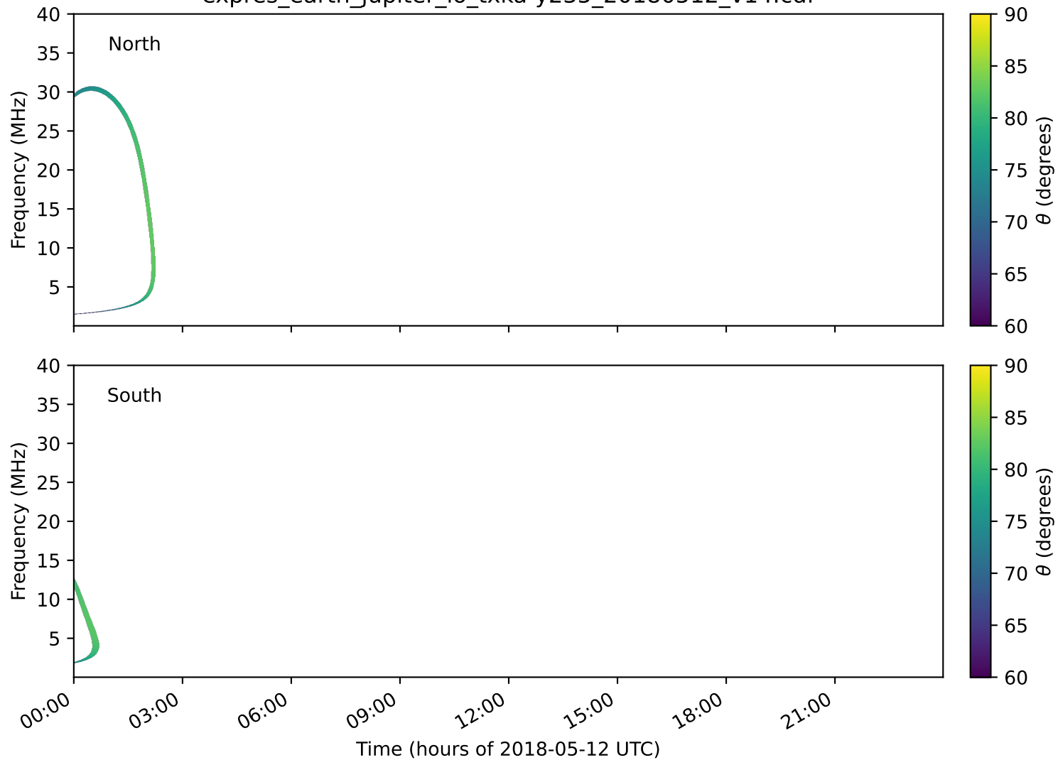
expres_earth_jupiter_io_txka-y235_20180512_v14.cdf
