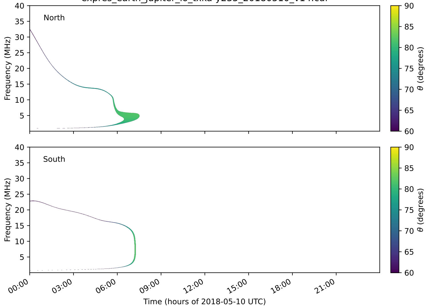
expres_earth_jupiter_io_txka-y235_20180510_v14.cdf
