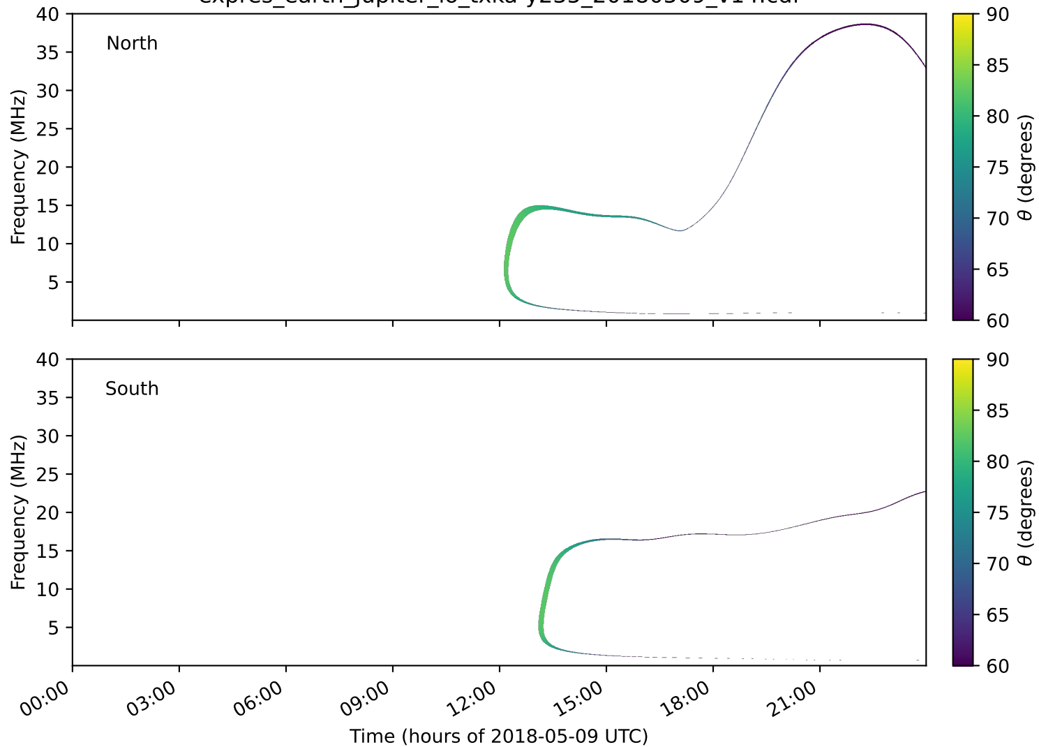
expres_earth_jupiter_io_txka-y235_20180509_v14.cdf
