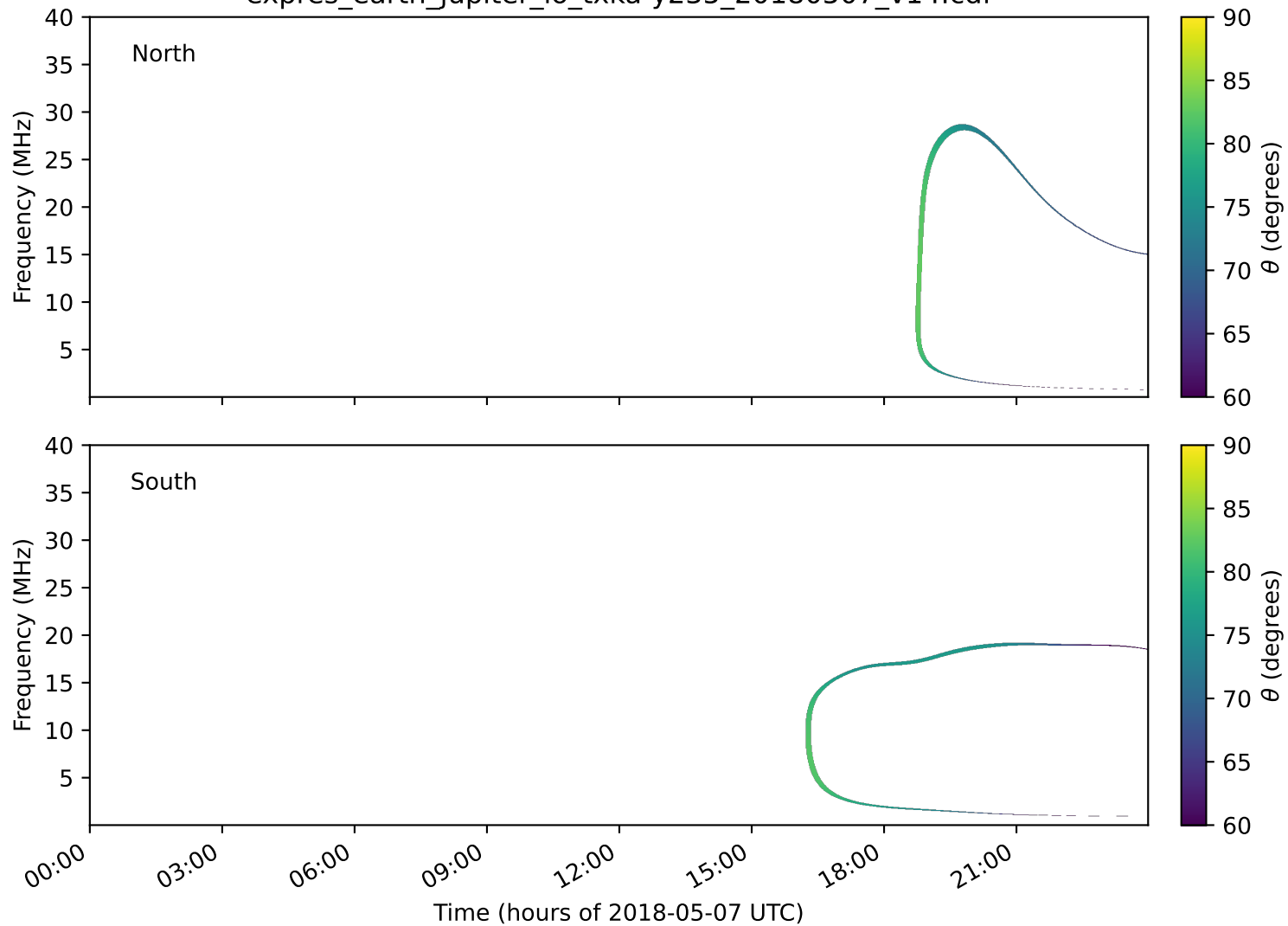
expres_earth_jupiter_io_txka-y235_20180507_v14.cdf
