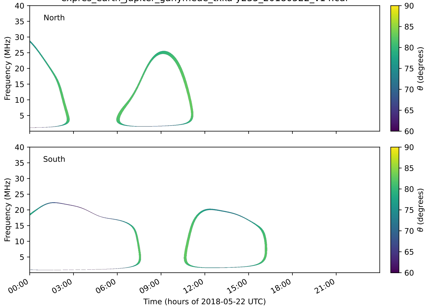
expres_earth_jupiter_ganymede_txka-y235_20180522_v14.cdf
