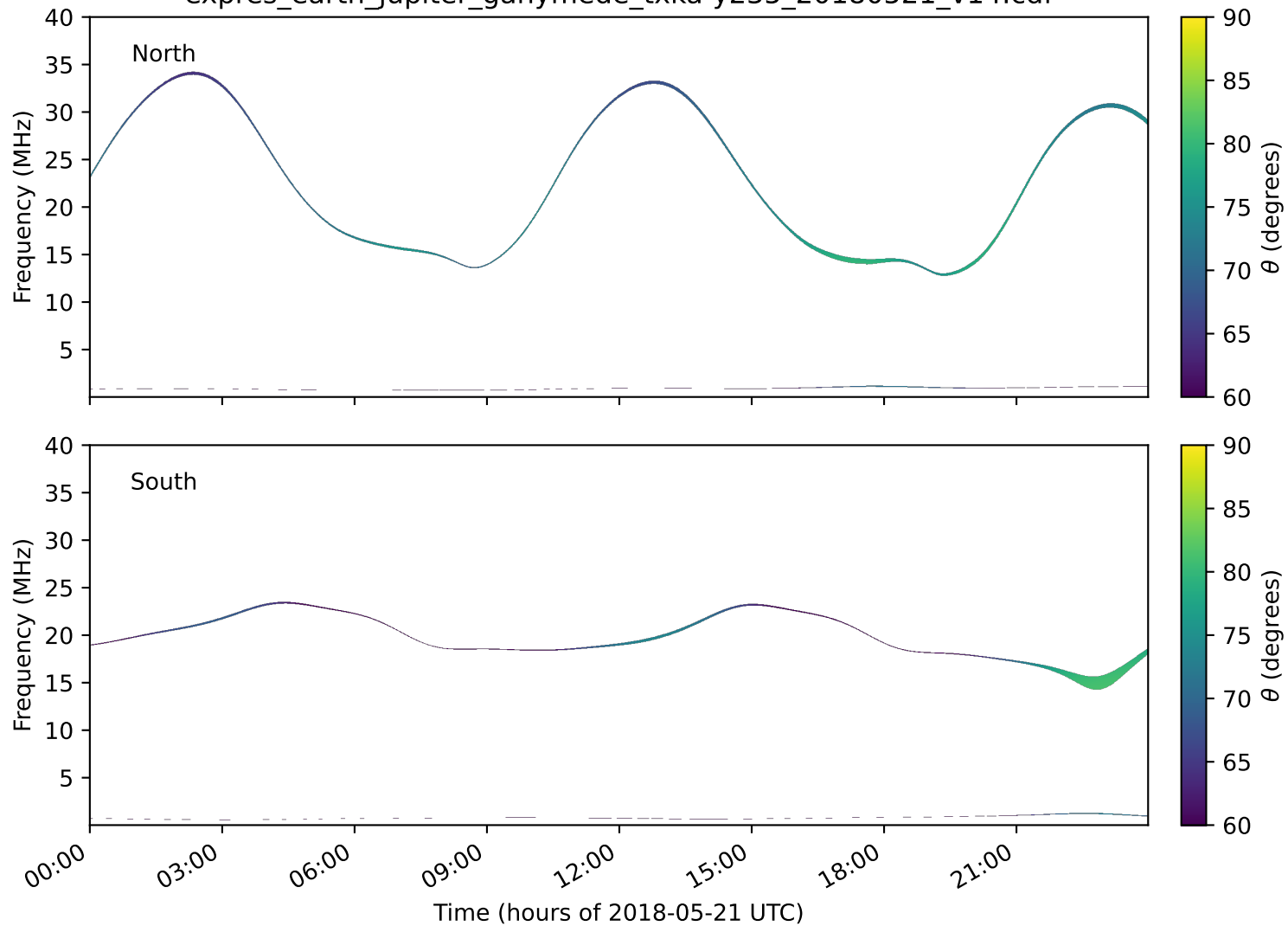
expres_earth_jupiter_ganymede_txka-y235_20180521_v14.cdf
