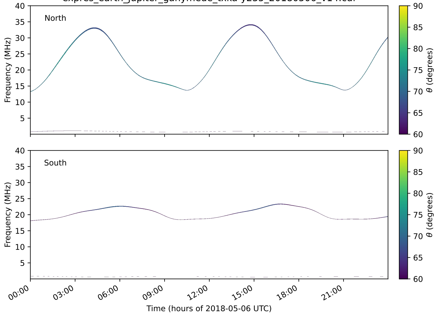
expres_earth_jupiter_ganymede_txka-y235_20180506_v14.cdf
