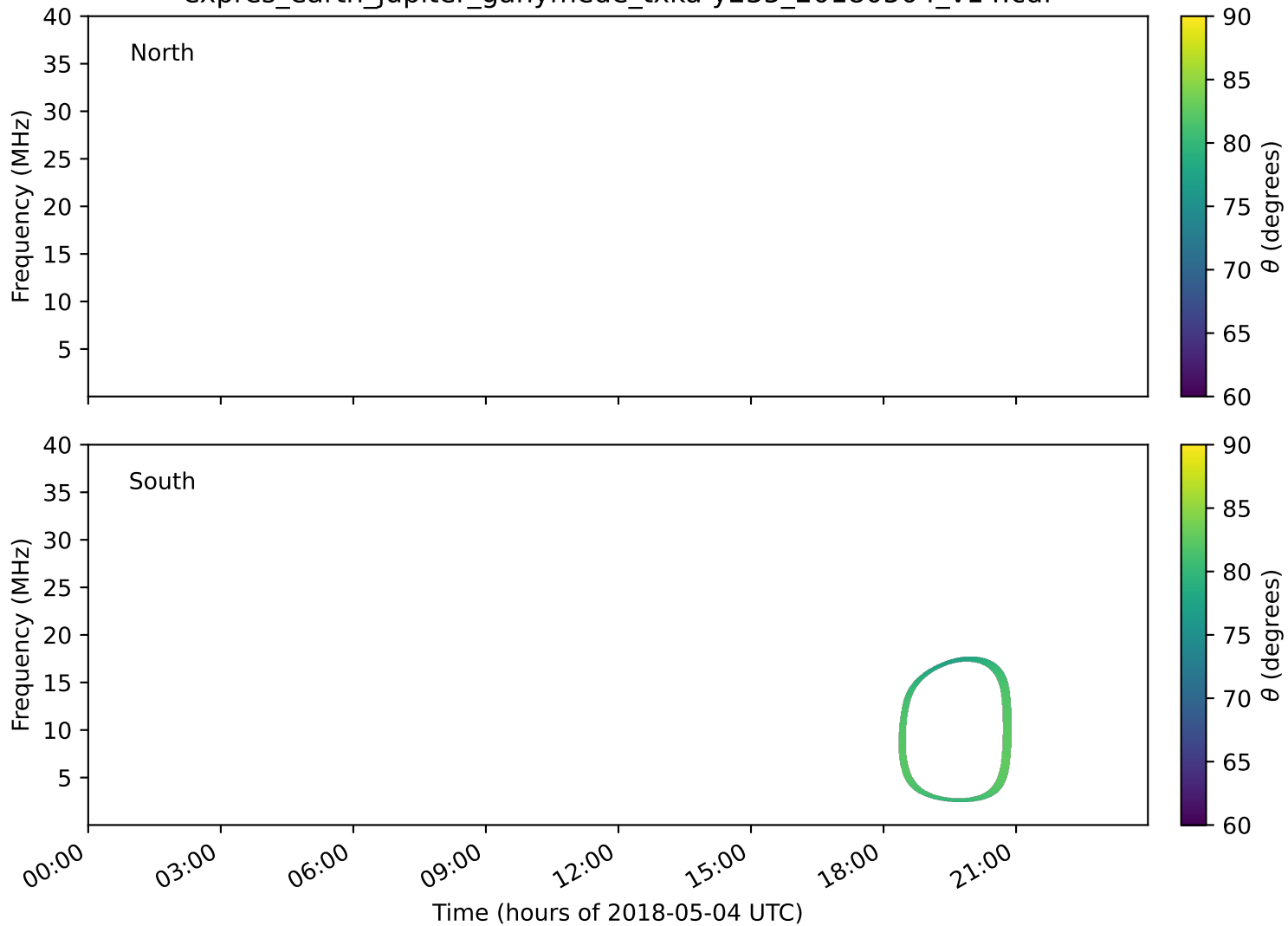
expres_earth_jupiter_ganymede_txka-y235_20180504_v14.cdf
