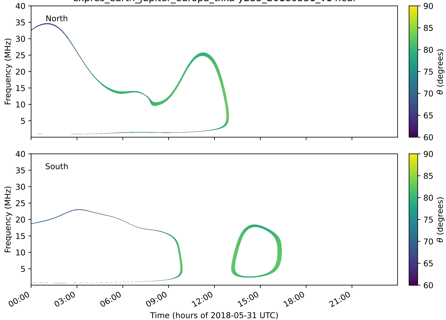
expres_earth_jupiter_europa_txka-y235_20180531_v14.cdf
