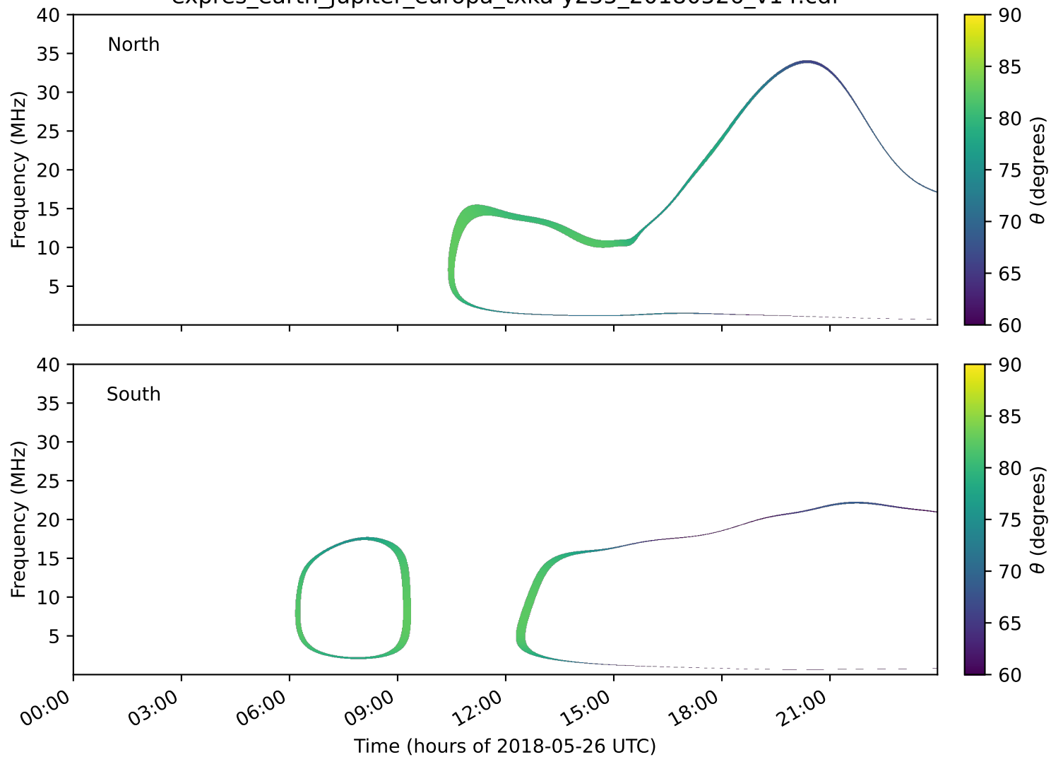
expres_earth_jupiter_europa_txka-y235_20180526_v14.cdf
