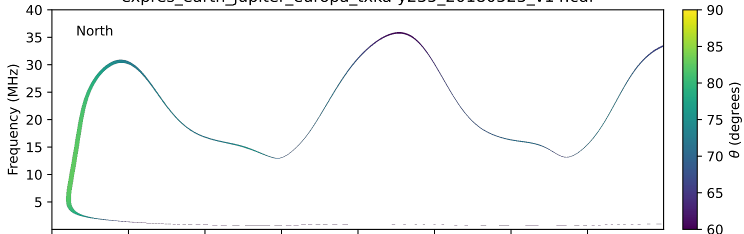
expres_earth_jupiter_europa_txka-y235_20180523_v14.cdf
