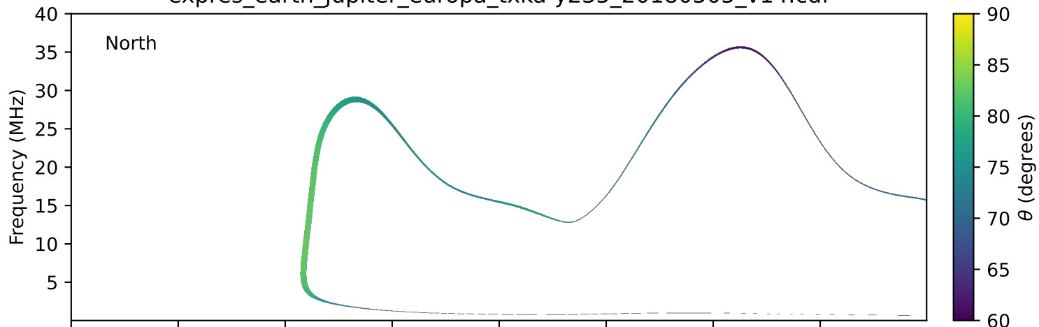
expres_earth_jupiter_europa_txka-y235_20180505_v14.cdf
