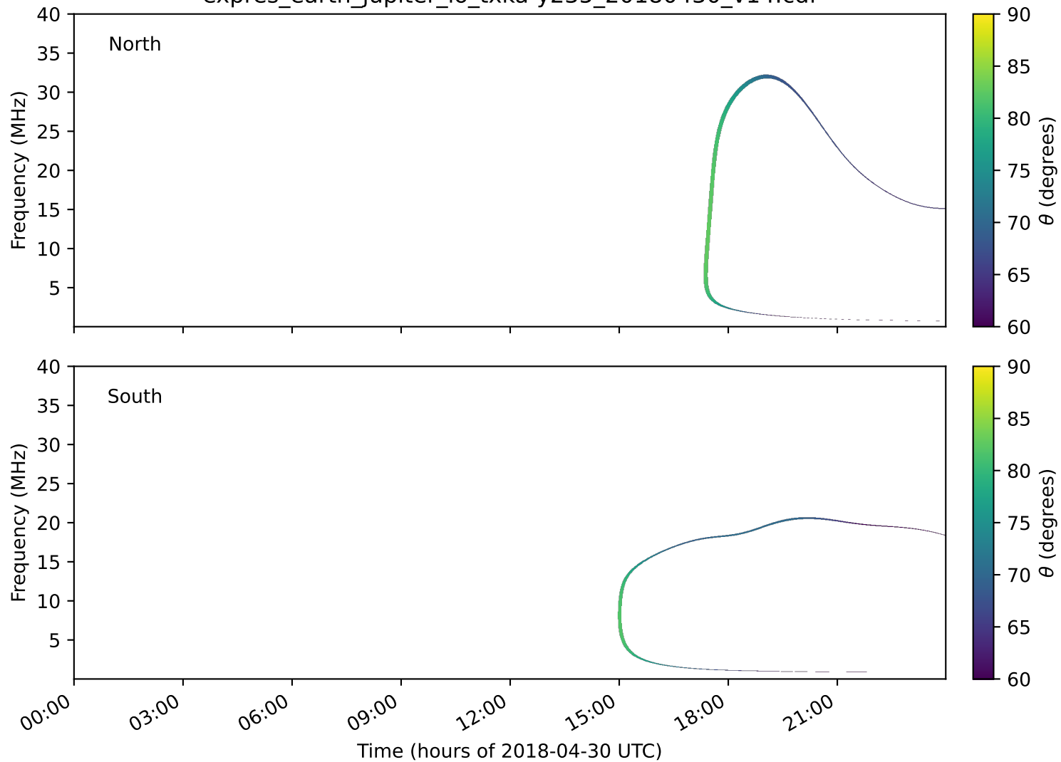
expres_earth_jupiter_io_txka-y235_20180430_v14.cdf
