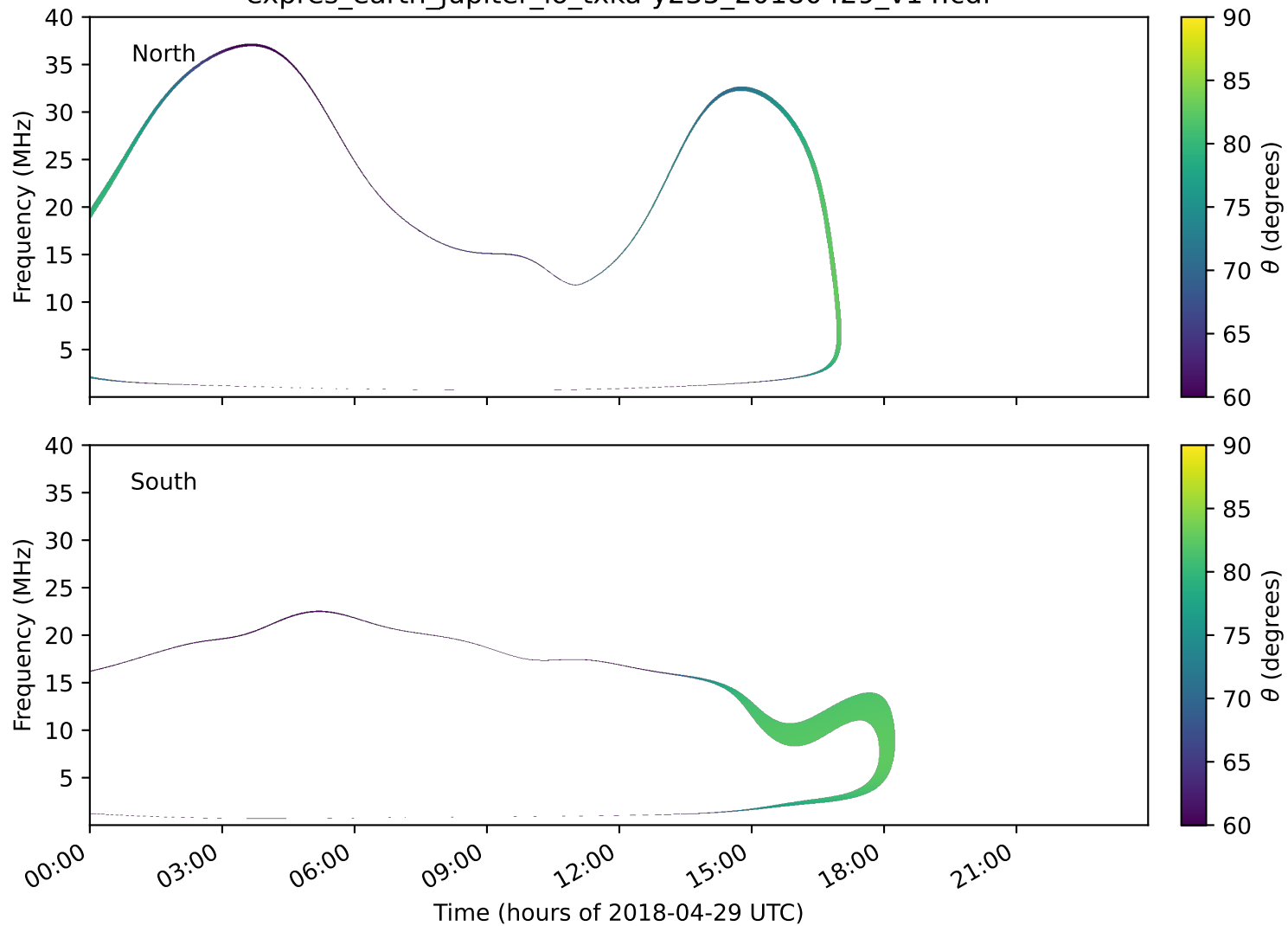
expres_earth_jupiter_io_txka-y235_20180429_v14.cdf
