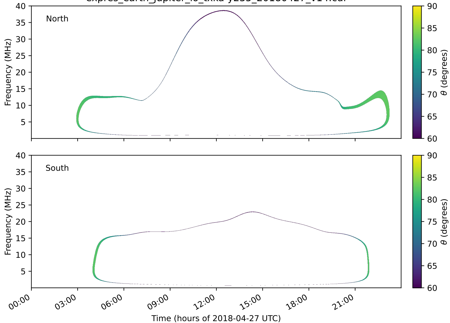
expres_earth_jupiter_io_txka-y235_20180427_v14.cdf
