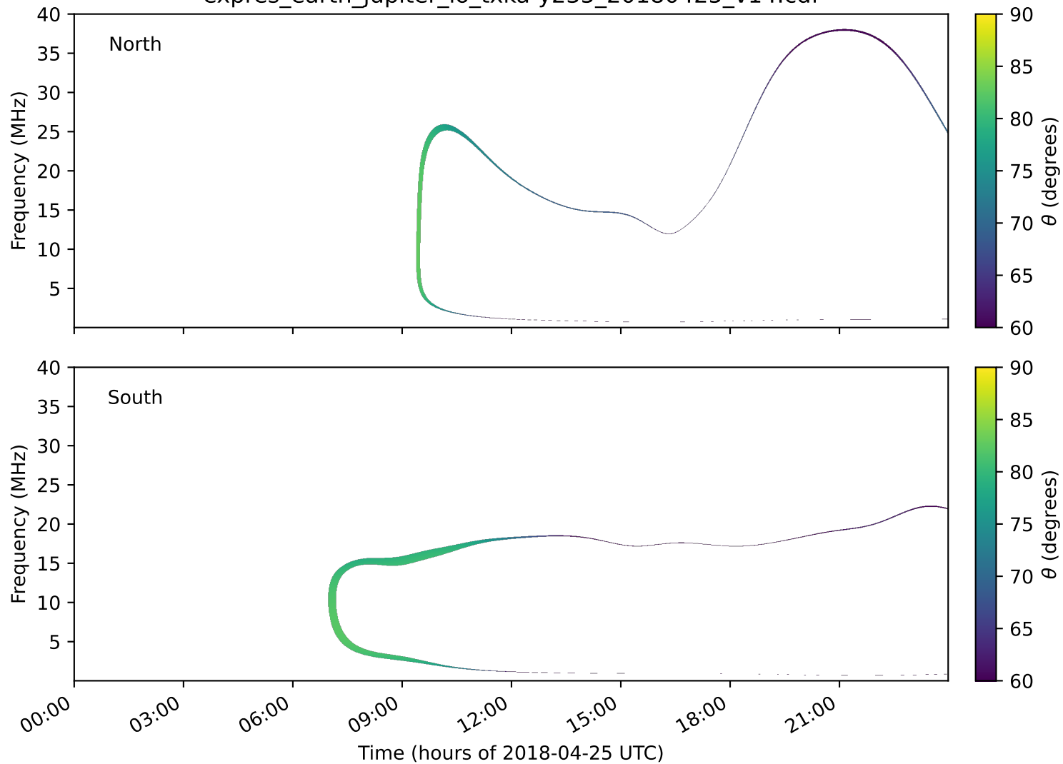
expres_earth_jupiter_io_txka-y235_20180425_v14.cdf
