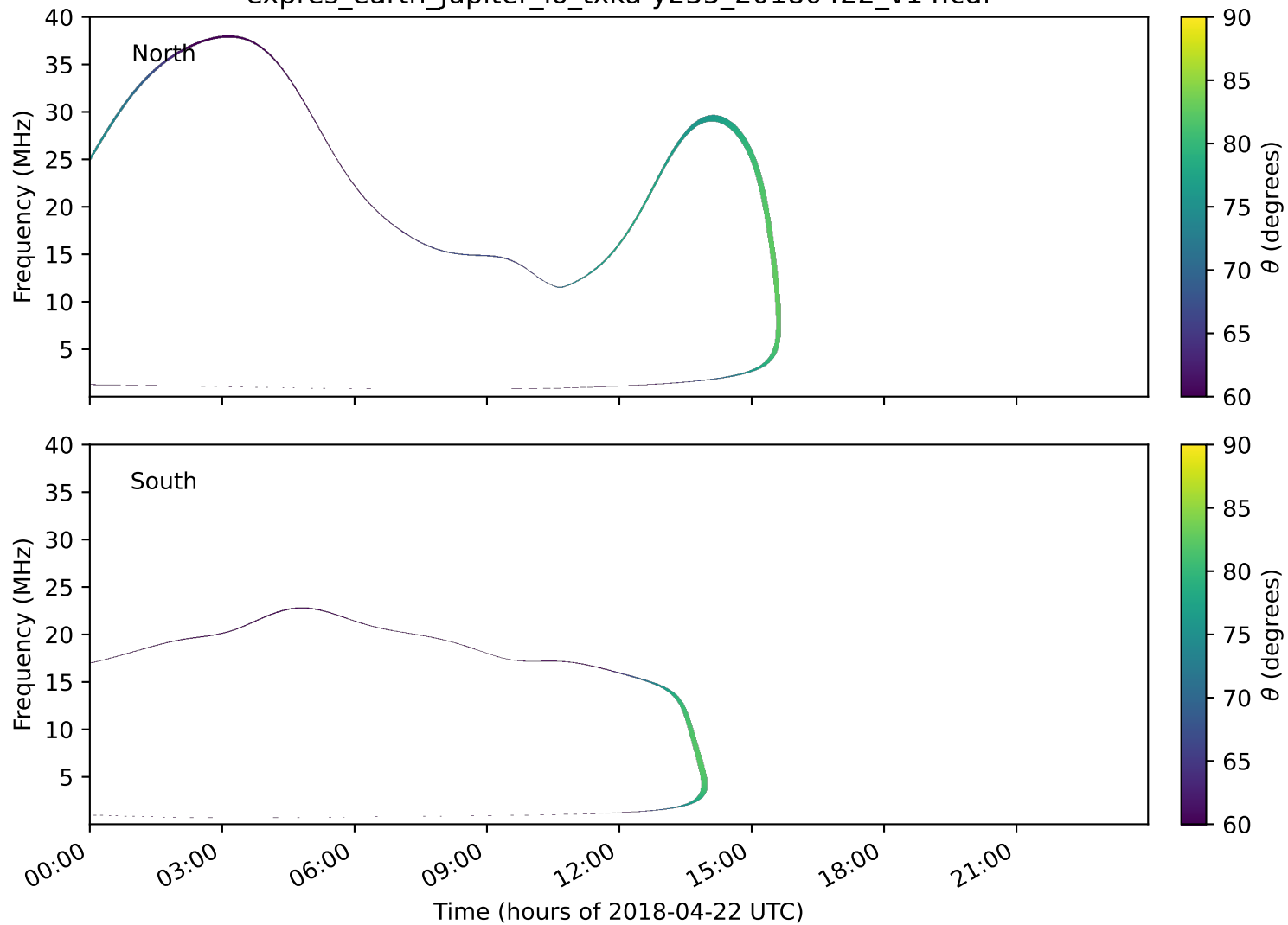
expres_earth_jupiter_io_txka-y235_20180422_v14.cdf
