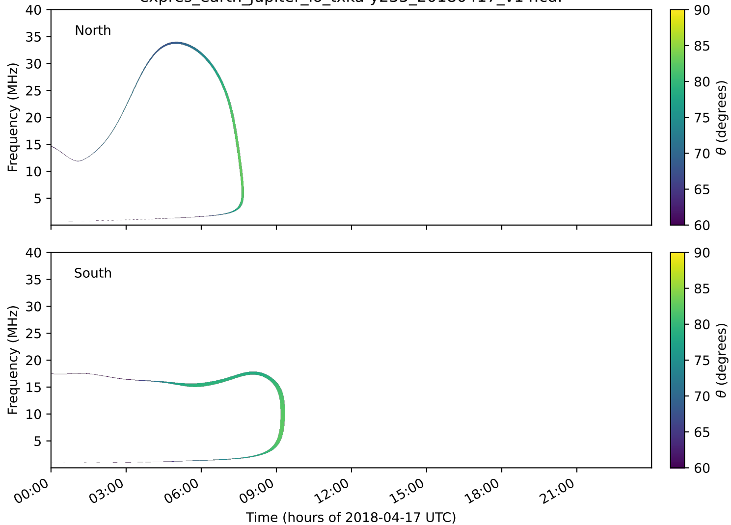
expres_earth_jupiter_io_txka-y235_20180417_v14.cdf
