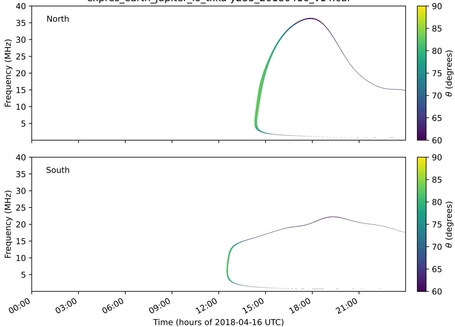
expres_earth_jupiter_io_txka-y235_20180416_v14.cdf
