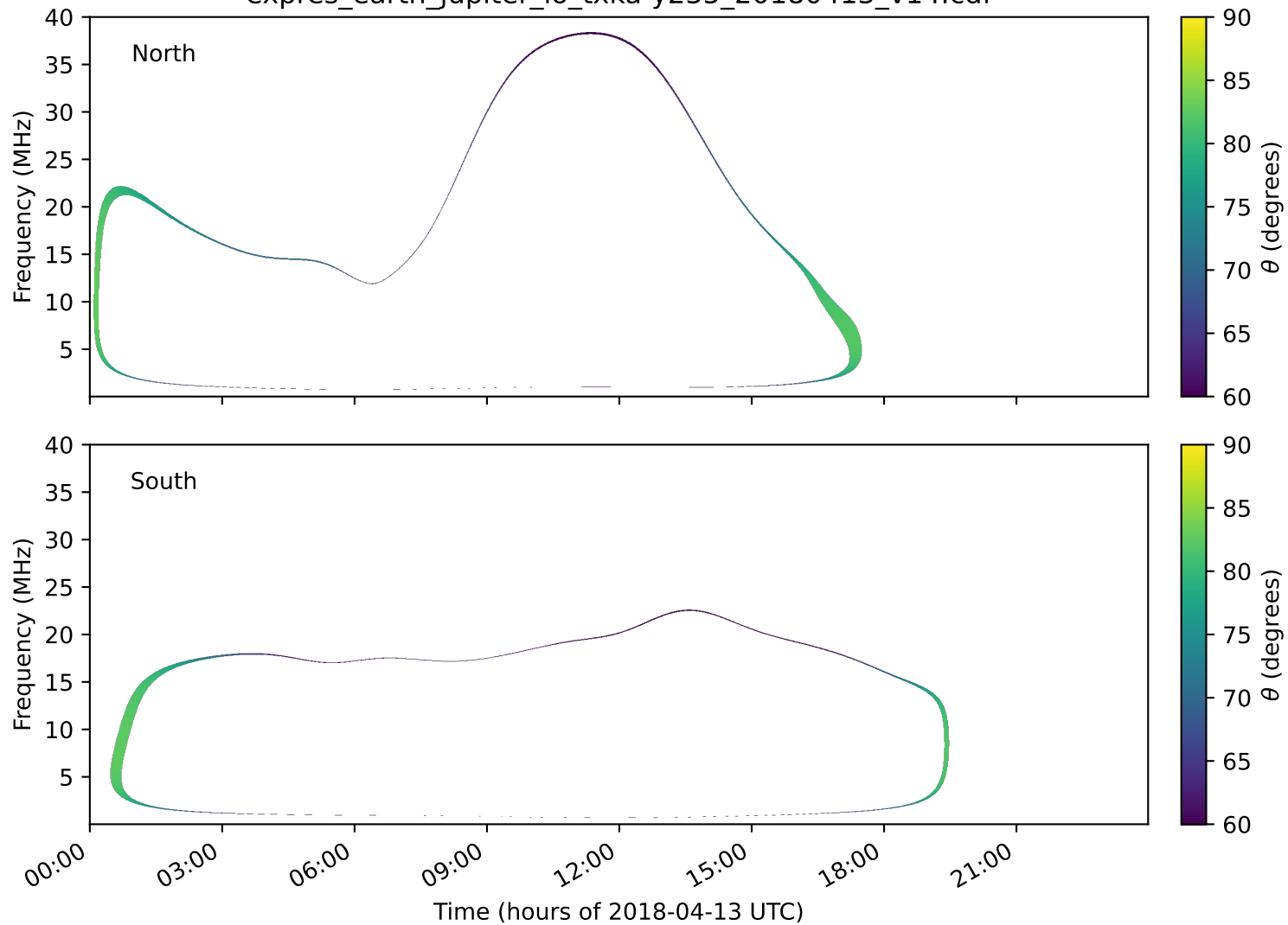
expres_earth_jupiter_io_txka-y235_20180413_v14.cdf
