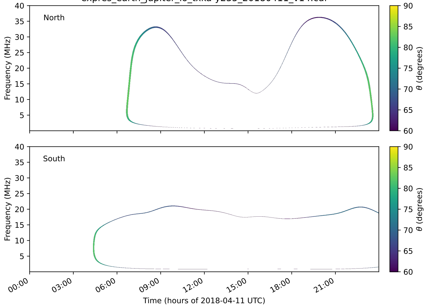
expres_earth_jupiter_io_txka-y235_20180411_v14.cdf
