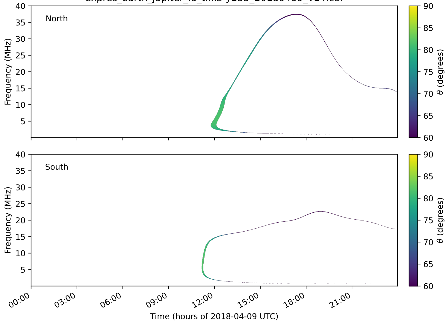
expres_earth_jupiter_io_txka-y235_20180409_v14.cdf
