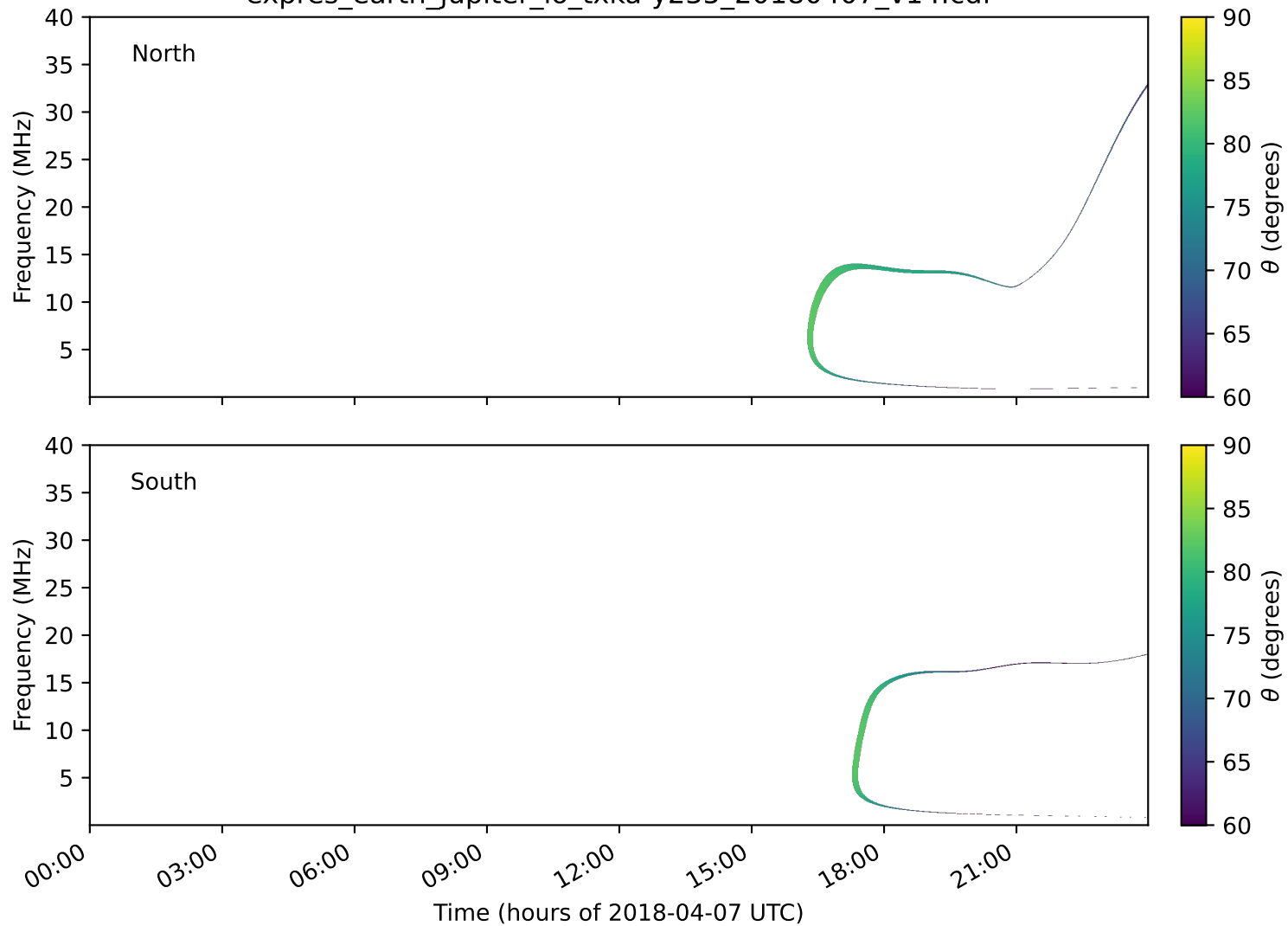
expres_earth_jupiter_io_txka-y235_20180407_v14.cdf
