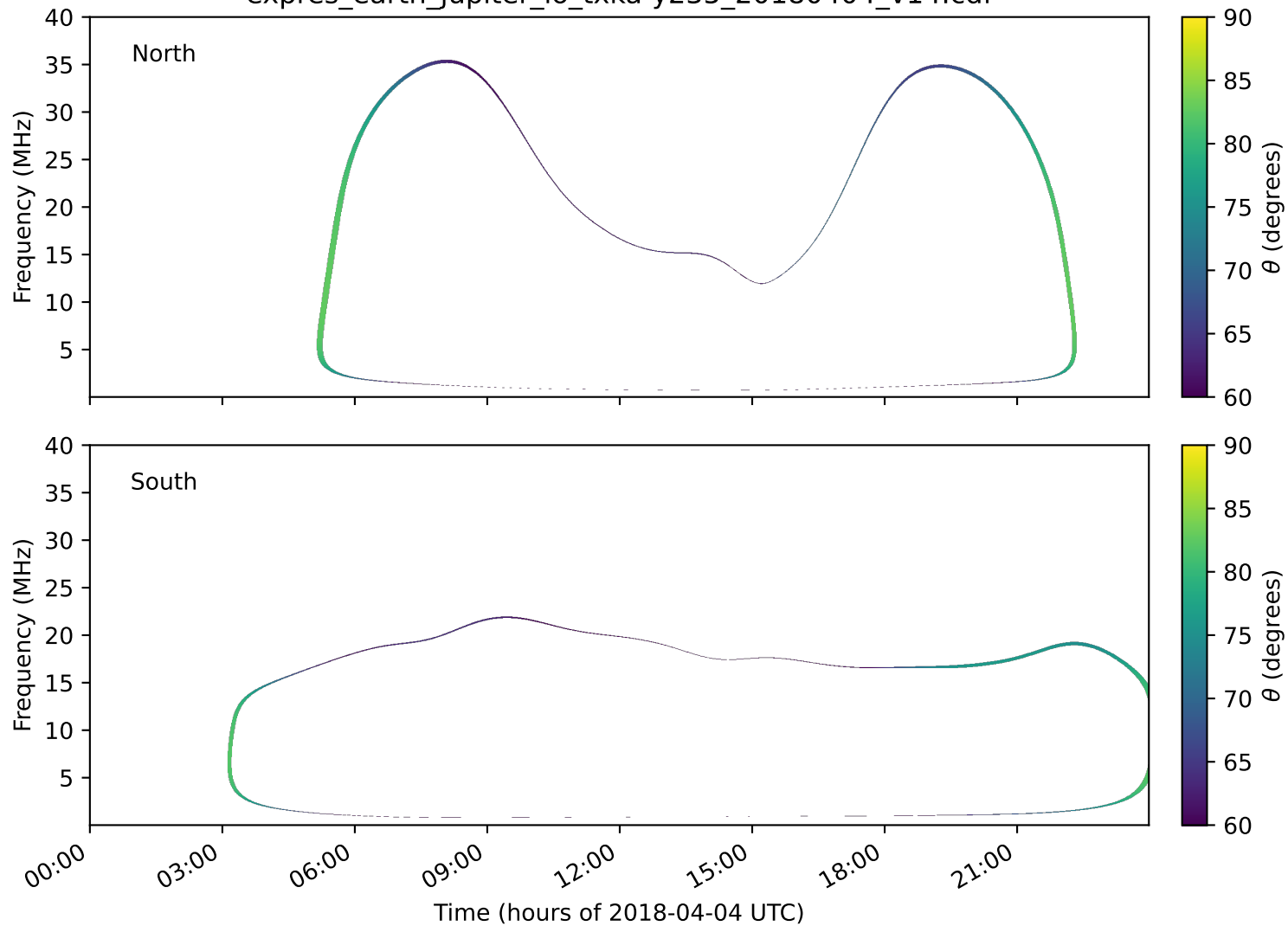
expres_earth_jupiter_io_txka-y235_20180404_v14.cdf
