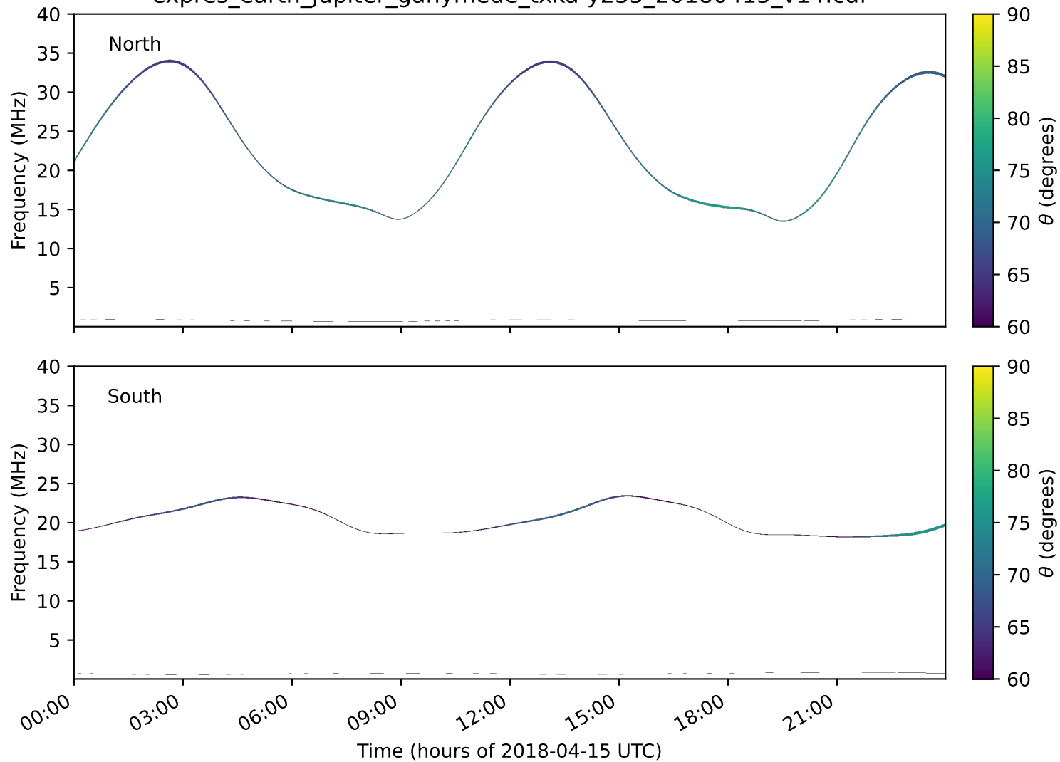
expres_earth_jupiter_ganymede_txka-y235_20180415_v14.cdf
