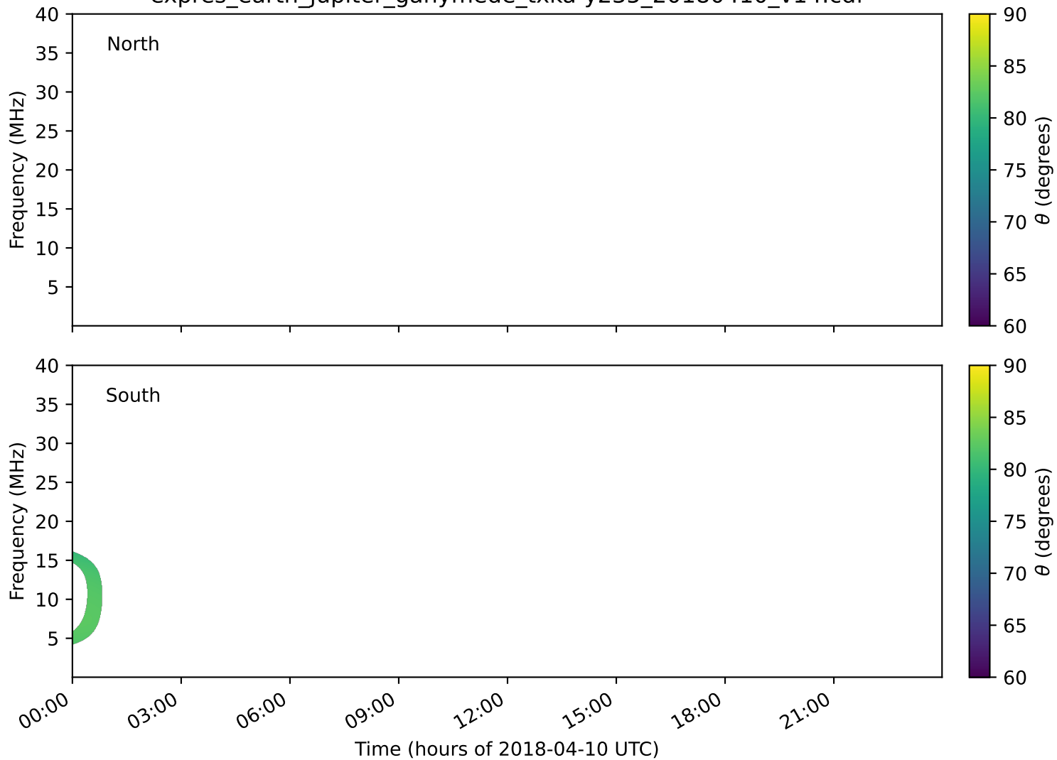
expres_earth_jupiter_ganymede_txka-y235_20180410_v14.cdf
