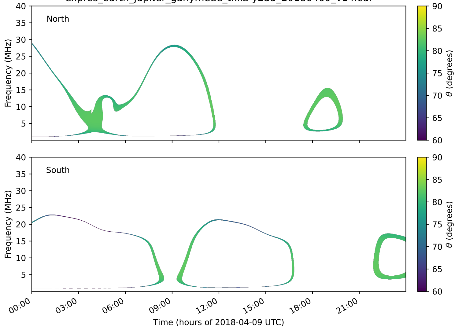
expres_earth_jupiter_ganymede_txka-y235_20180409_v14.cdf
