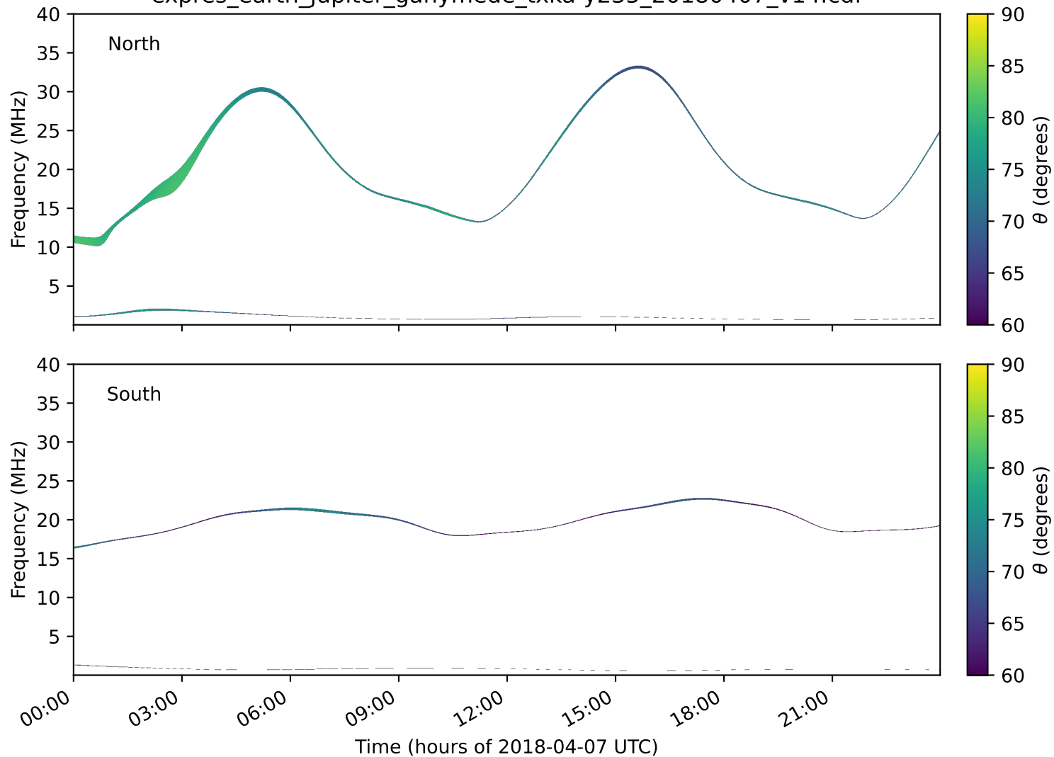
expres_earth_jupiter_ganymede_txka-y235_20180407_v14.cdf
