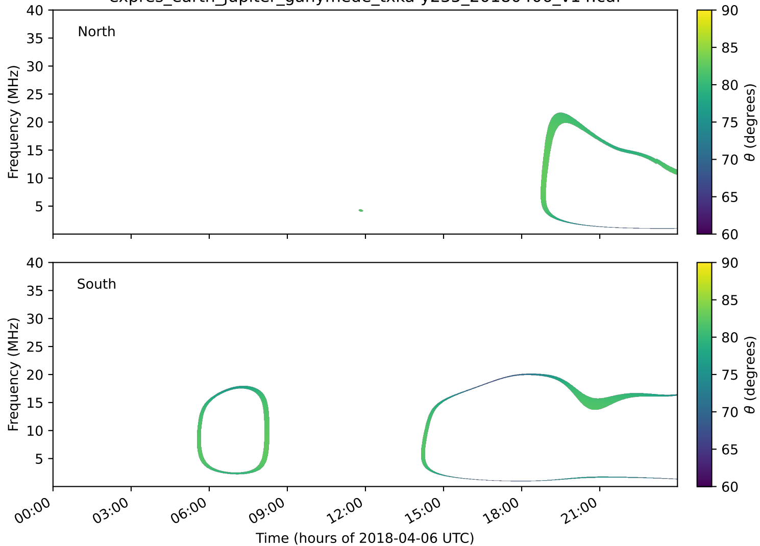
expres_earth_jupiter_ganymede_txka-y235_20180406_v14.cdf
