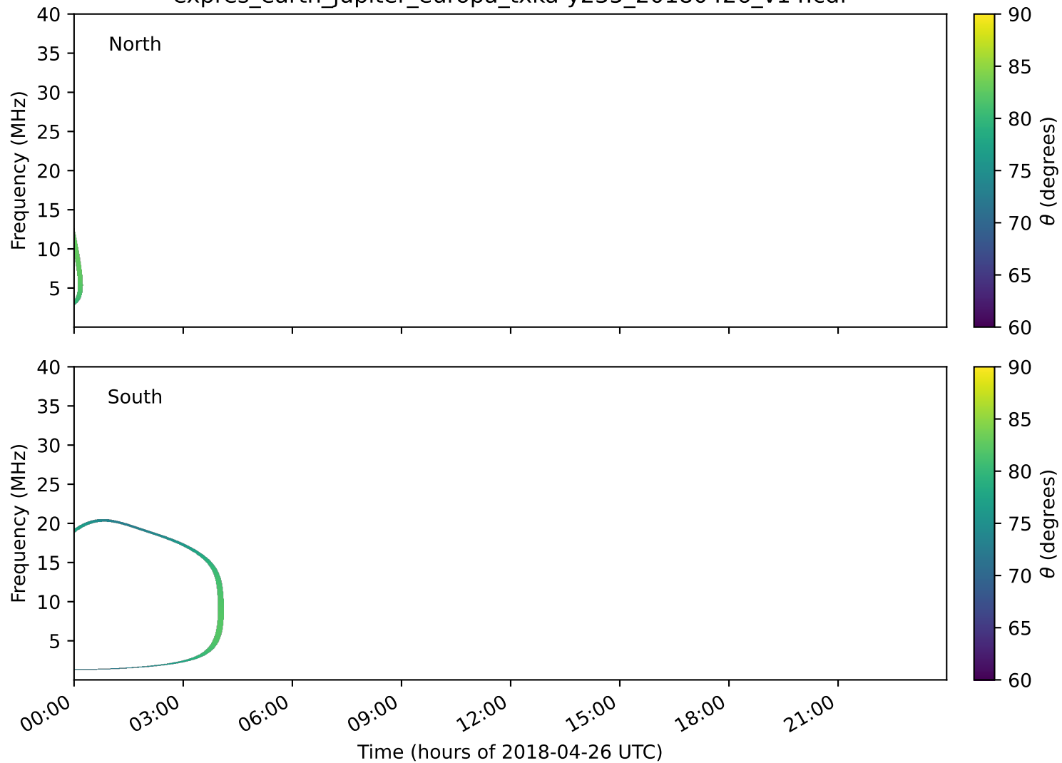
expres_earth_jupiter_europa_txka-y235_20180426_v14.cdf
